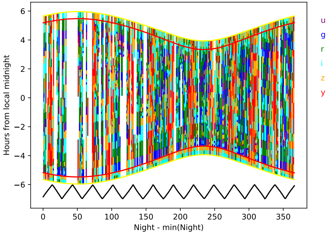
too_elab_r8_d3_griz_v3.4_10yrs year 8-9: Hourglass
