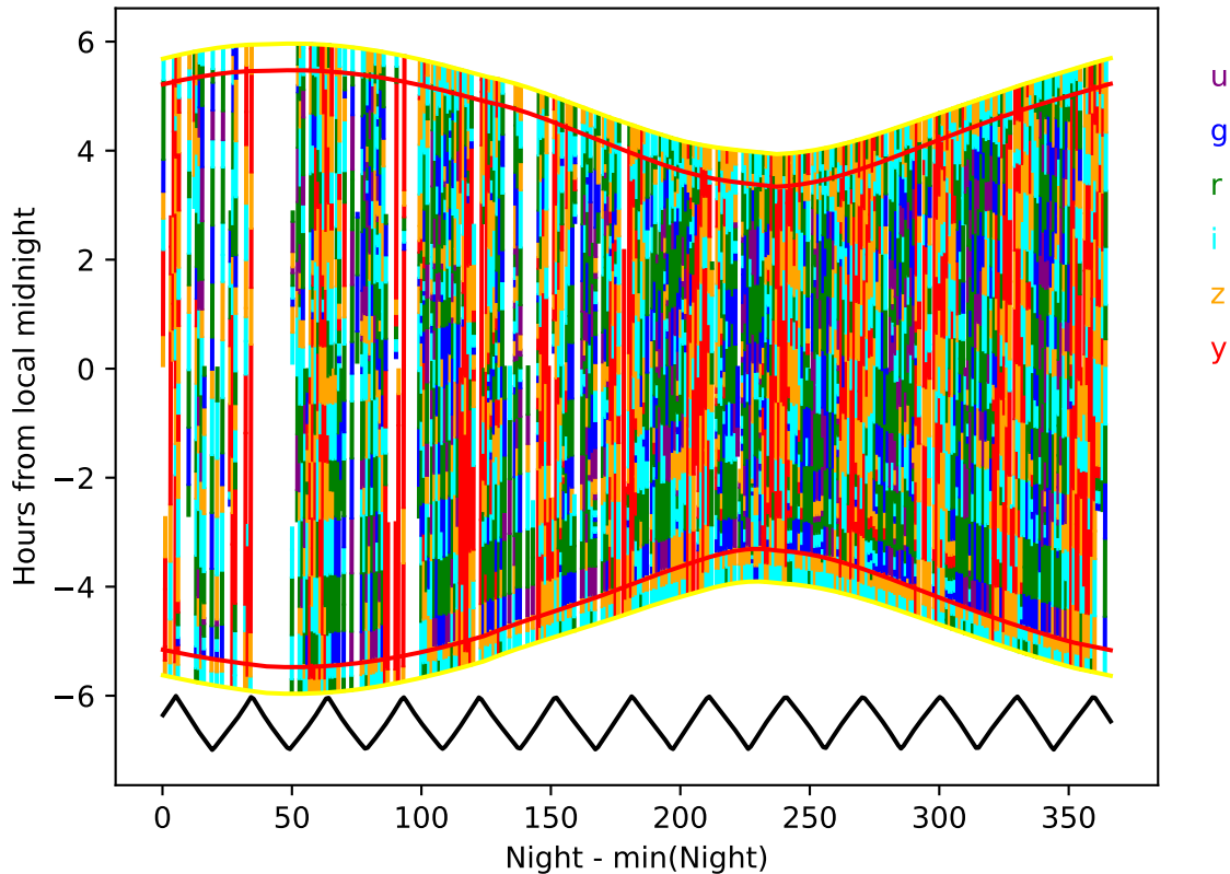
too_elab_r8_d3_griz_v3.4_10yrs year 6-7: Hourglass
