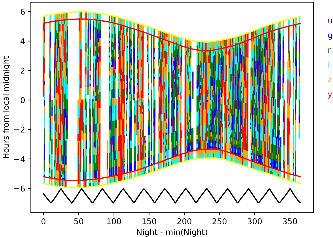
too_elab_r8_d3_griz_v3.4_10yrs year 4-5: Hourglass
