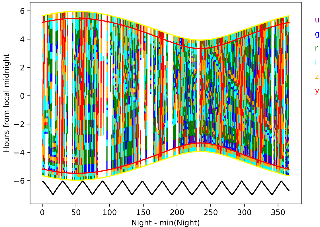
too_elab_r8_d3_griz_v3.4_10yrs year 1-2: Hourglass
