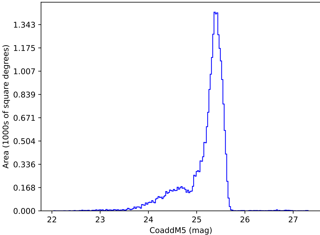
too_elab_r8_d3_griz_v3.4_10yrs u: CoaddM5
