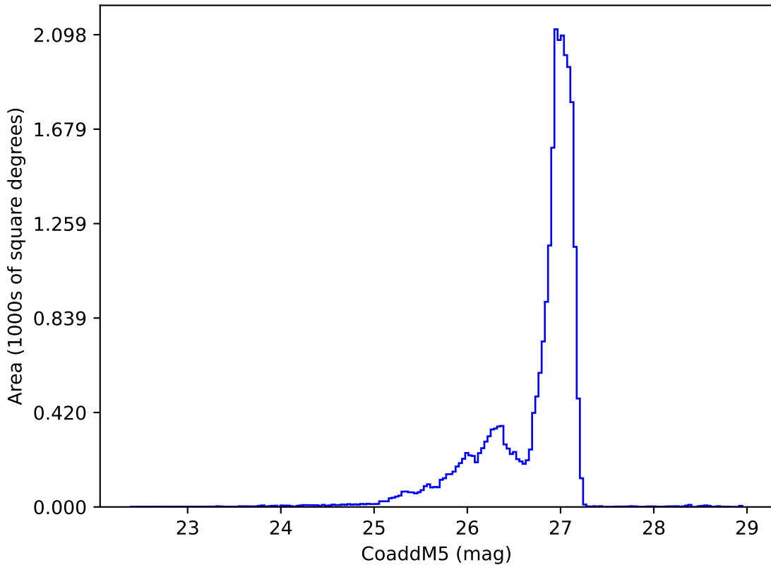
too_elab_r8_d3_griz_v3.4_10yrs r: CoaddM5
