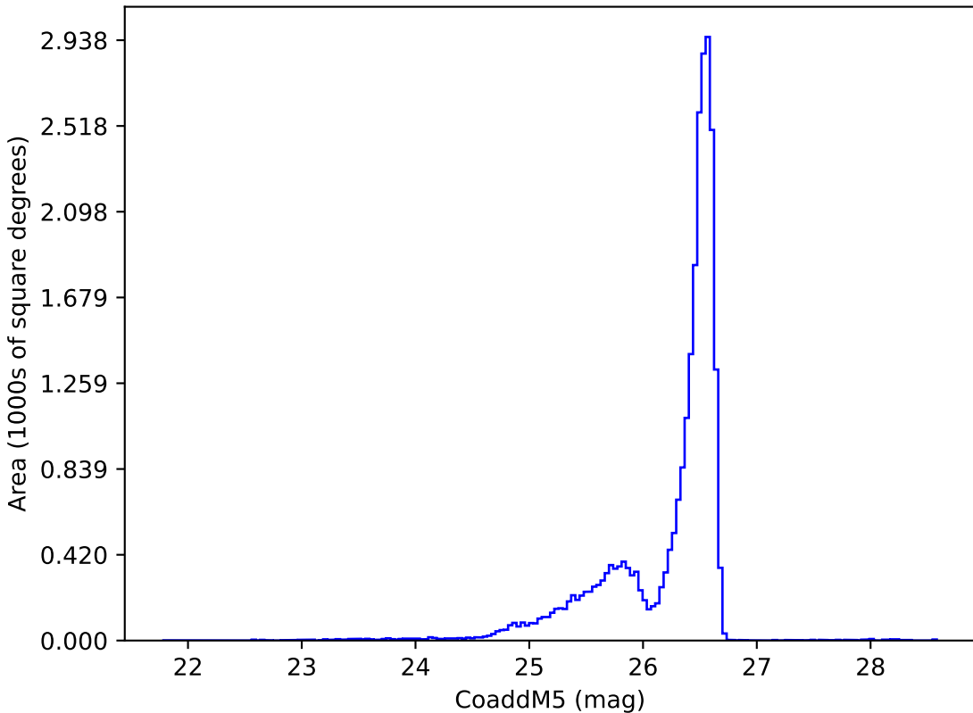
too_elab_r8_d3_griz_v3.4_10yrs i: CoaddM5
