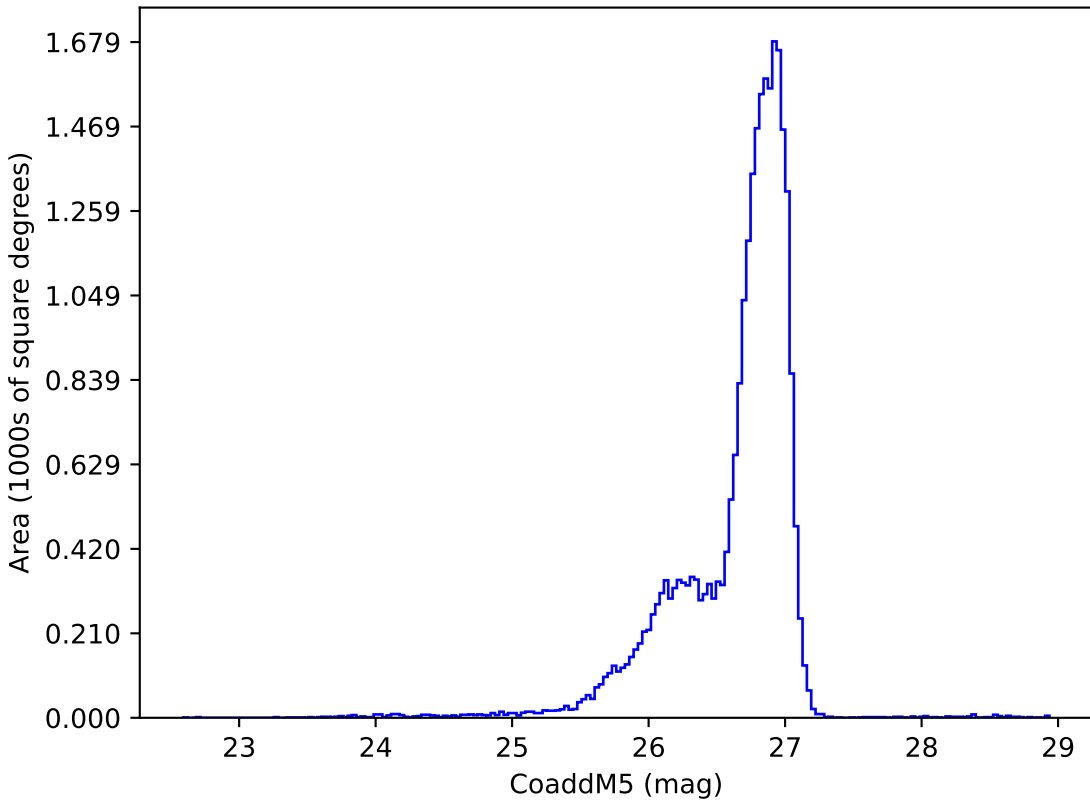
too_elab_r8_d3_griz_v3.4_10yrs g: CoaddM5
