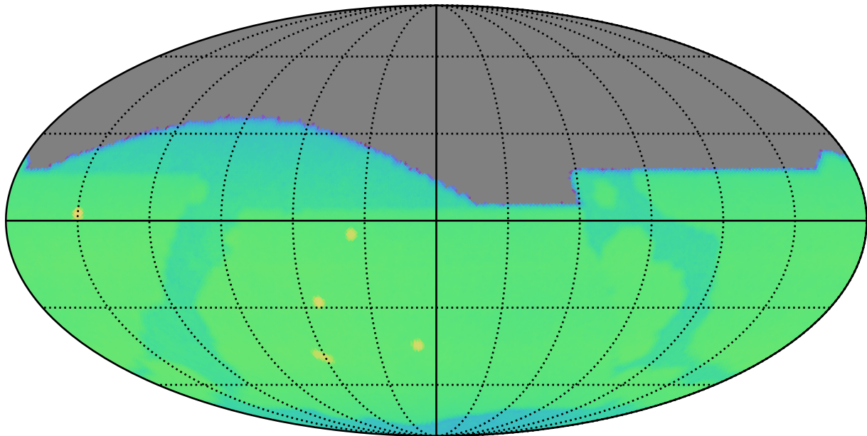
too_elab_r8_d3_griz_v3.4_10yrs : CoaddM5
