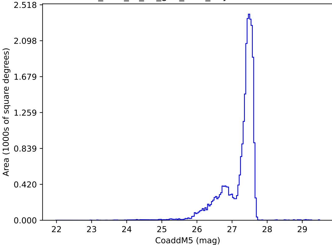
too_elab_r8_d3_griz_v3.4_10yrs : CoaddM5
