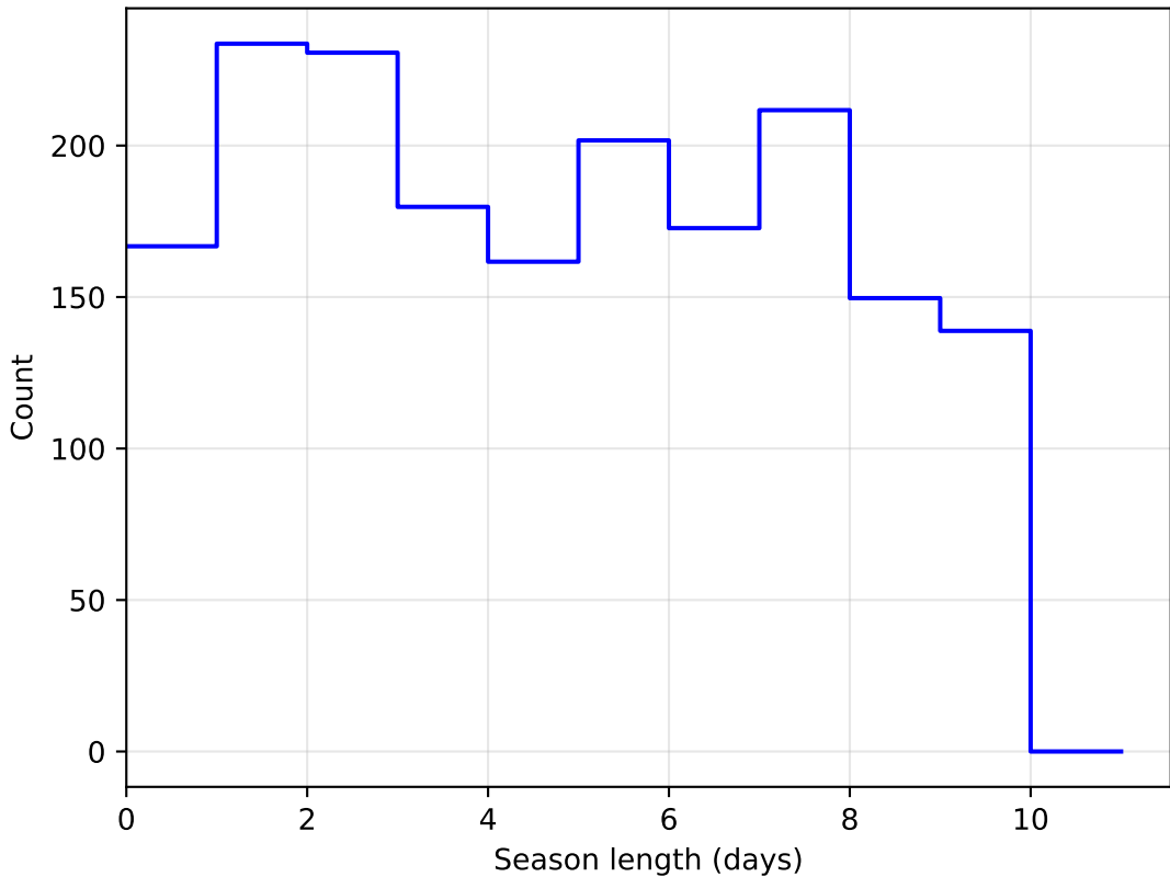
too_elab_r8_d3_griz_v3.4_10yrs DD:WFD all bands: SeasonLength
