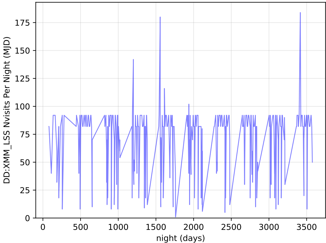
too_elab_r8_d3_griz_v3.4_10yrs all bands: DD:XMM_LSS Nvisits Per Night
