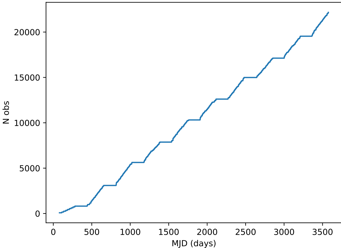
too_elab_r8_d3_griz_v3.4_10yrs all bands: DD:XMM_LSS Cumulative NVisits
