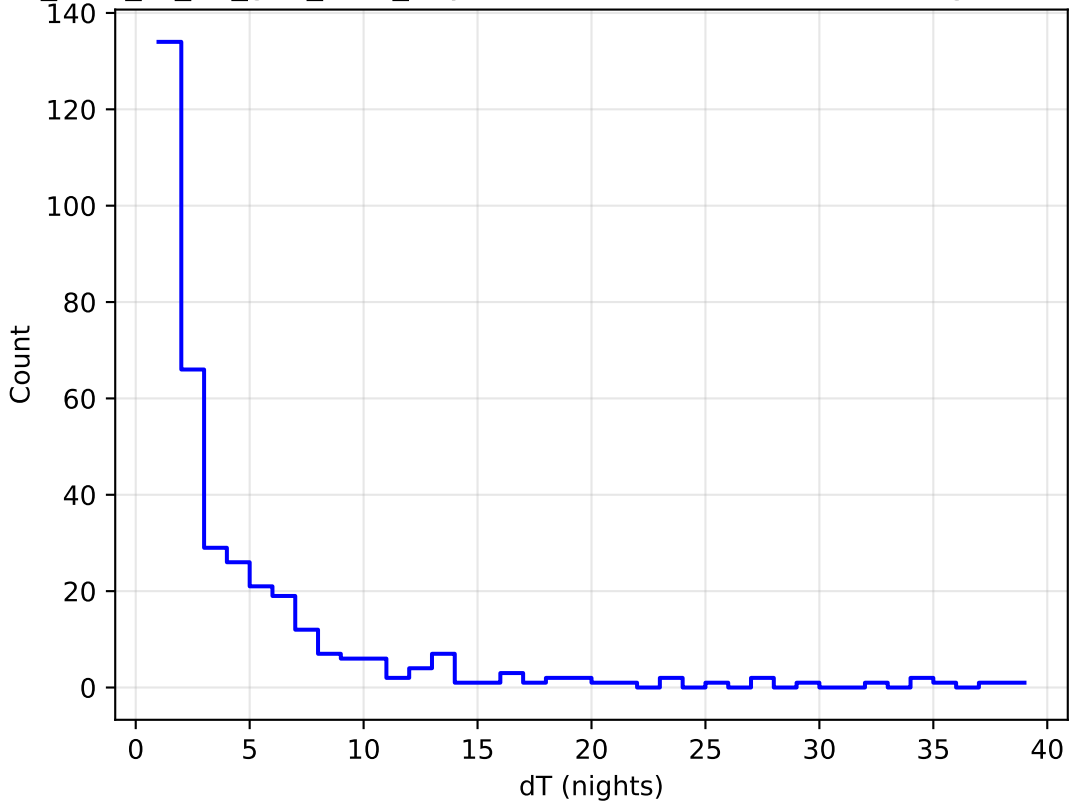
too_elab_r8_d3_griz_v3.4_10yrs all bands: DD:WFD Delta Nights Histogram
