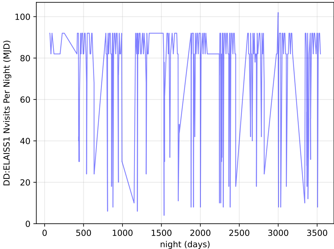
too_elab_r8_d3_griz_v3.4_10yrs all bands: DD:ELAISS1 Nvisits Per Night
