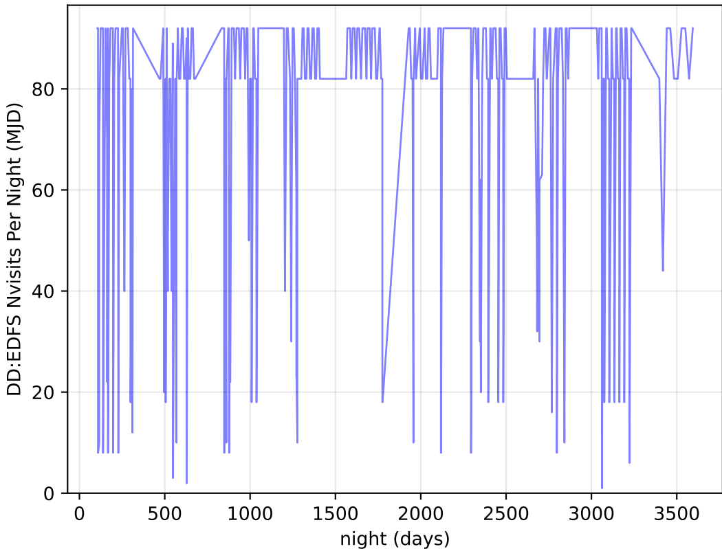
too_elab_r8_d3_griz_v3.4_10yrs all bands: DD:EDFS Nvisits Per Night
