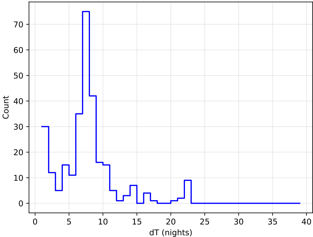
too_elab_r8_d3_griz_v3.4_10yrs all bands: DD:EDFS Delta Nights Histogram
