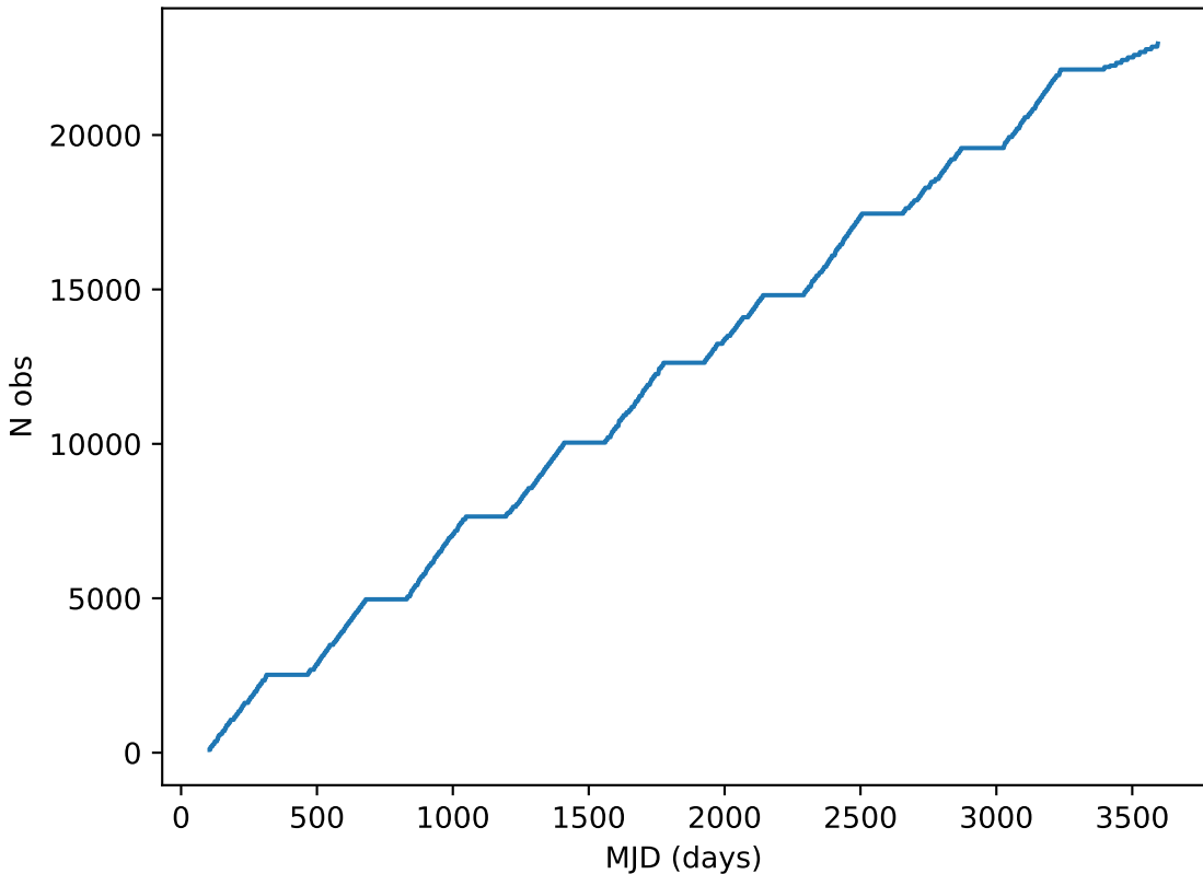
too_elab_r8_d3_griz_v3.4_10yrs all bands: DD:EDFS Cumulative NVisits
