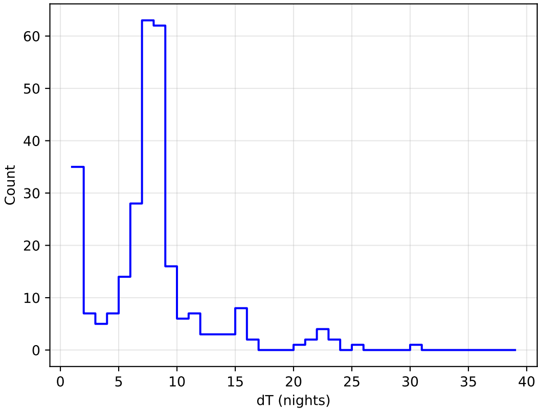
too_elab_r8_d3_griz_v3.4_10yrs all bands: DD:ECDFS Delta Nights Histogram
