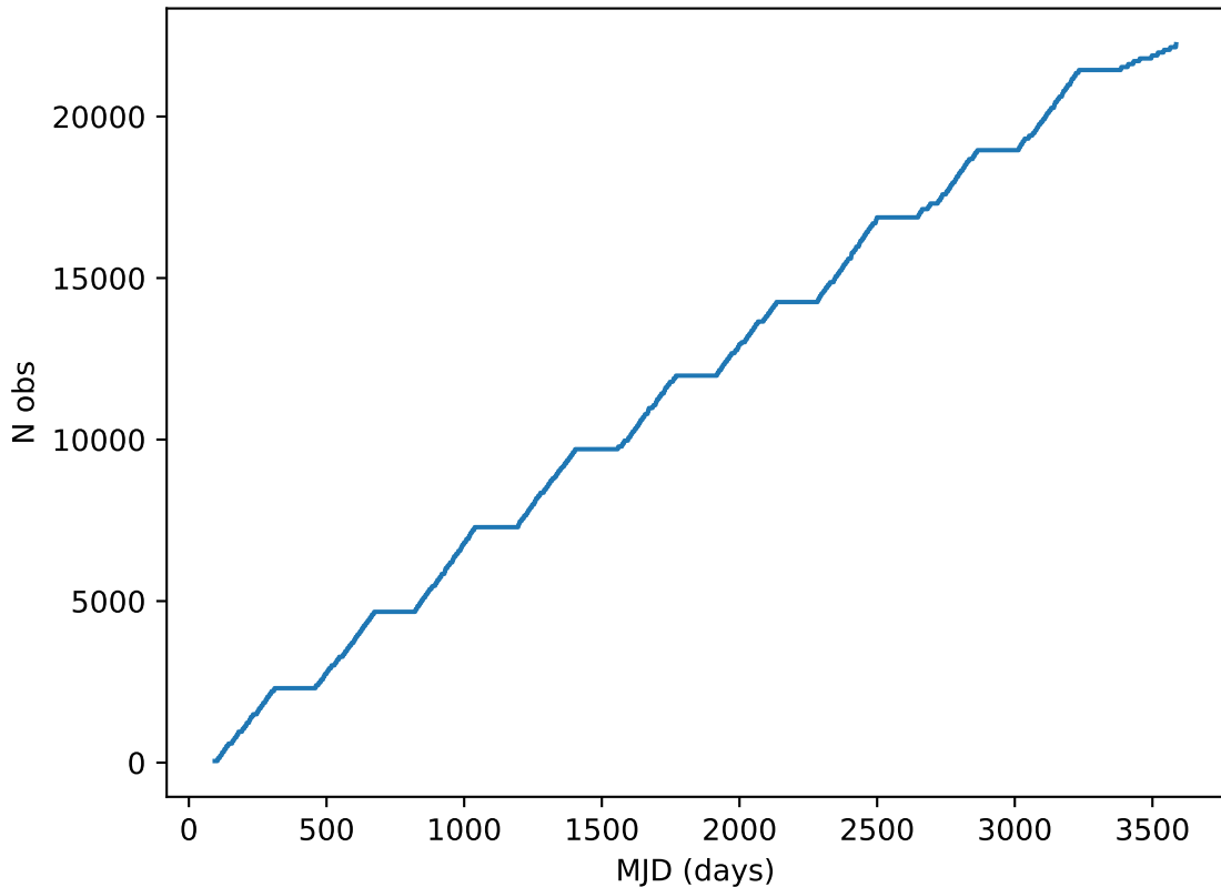
too_elab_r8_d3_griz_v3.4_10yrs all bands: DD:ECDFS Cumulative NVisits
