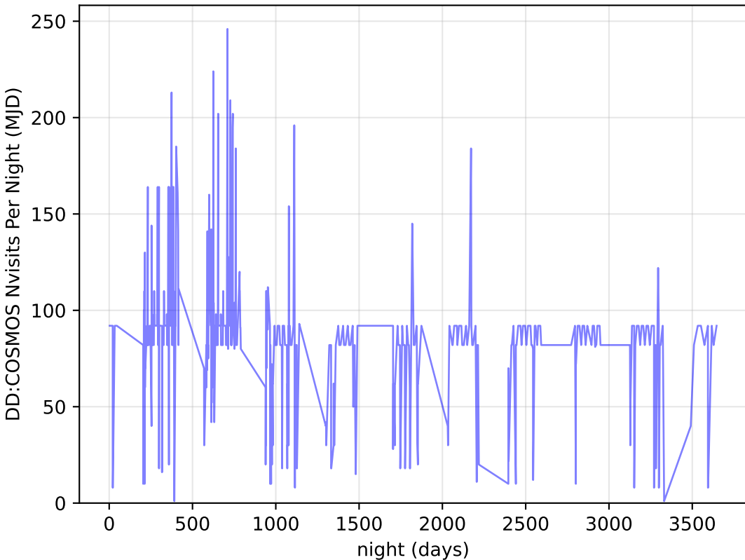
too_elab_r8_d3_griz_v3.4_10yrs all bands: DD: COSMOS Nvisits Per Night
