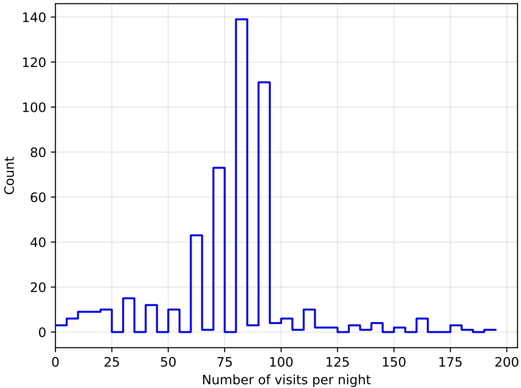
too_elab_r8_d3_griz_v3.4_10yrs all bands: DD: COSMOS NVisitsPerNight
