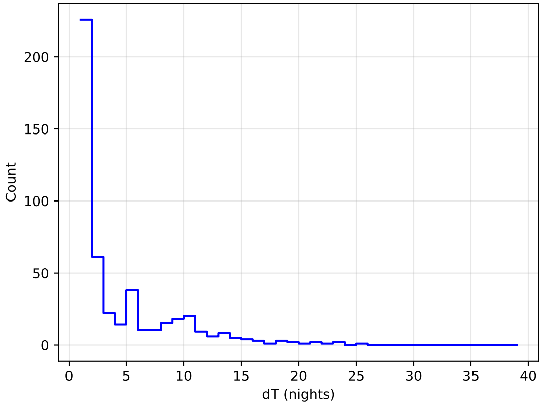
too_elab_r8_d3_griz_v3.4_10yrs all bands: DD:COSMOS Delta Nights Histogram
