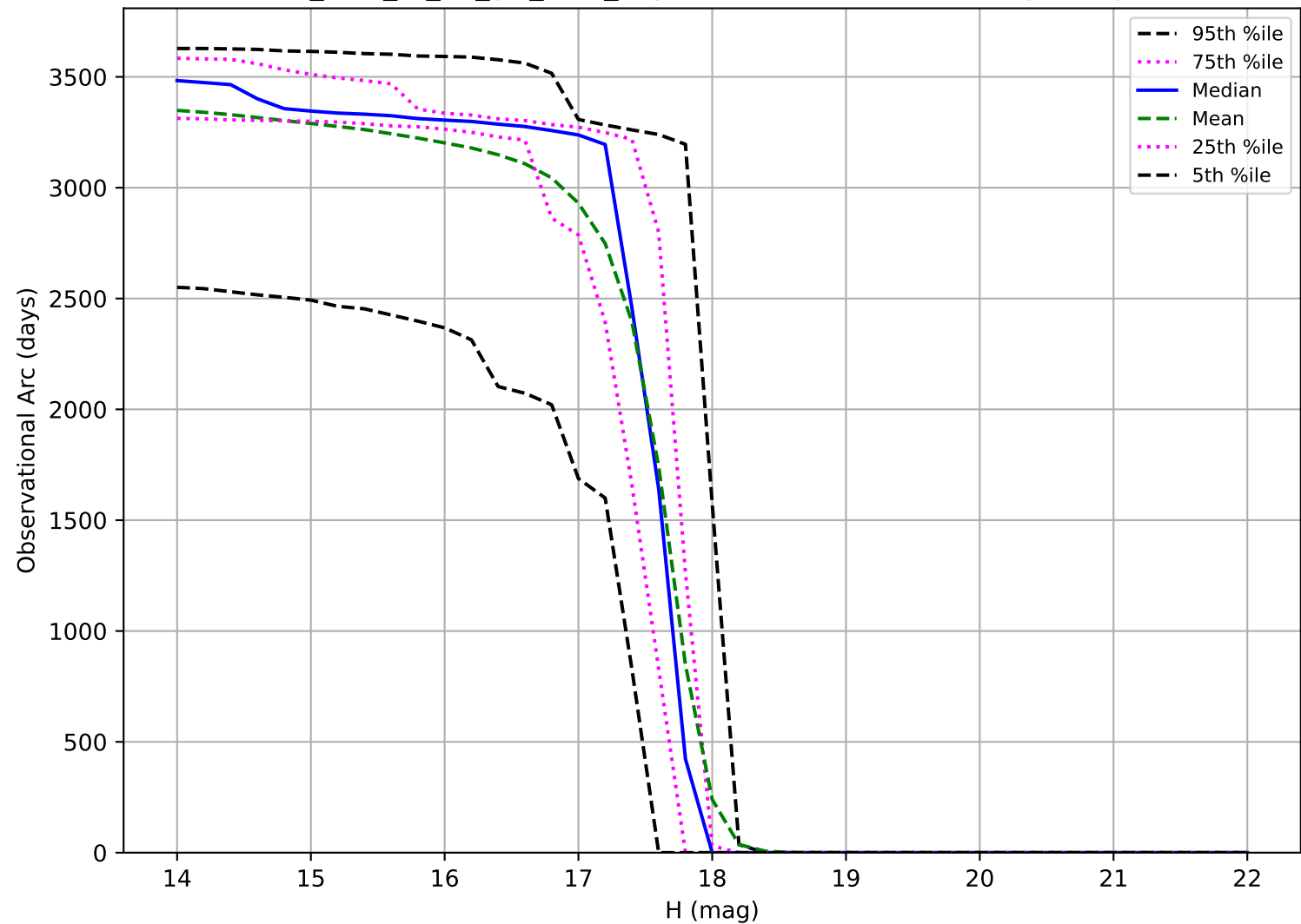
too_elab_r8_d3_giz_v3.4_10yrs: Observational Arc Length Trojan
