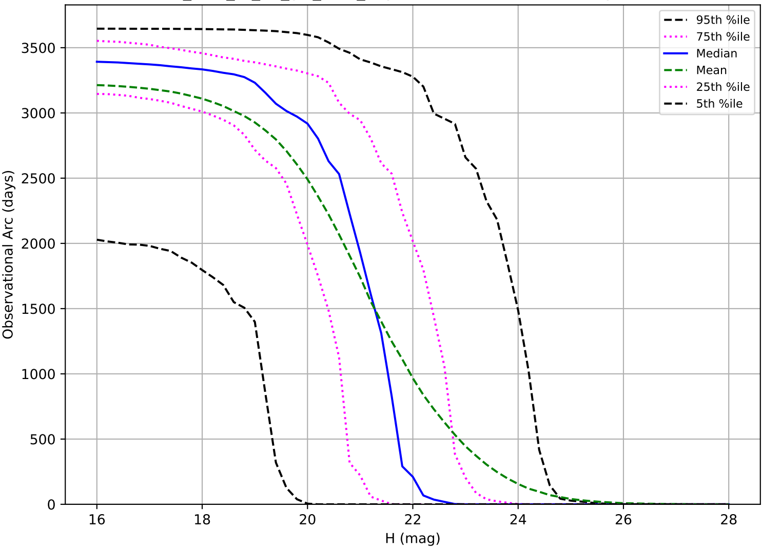
too_elab_r8_d3_giz_v3.4_10yrs: Observational Arc Length PHA
