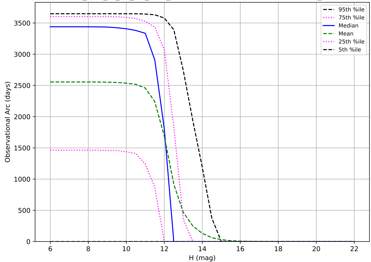
too_elab_r8_d3_giz_v3.4_10yrs: Observational Arc Length OCC_r20
