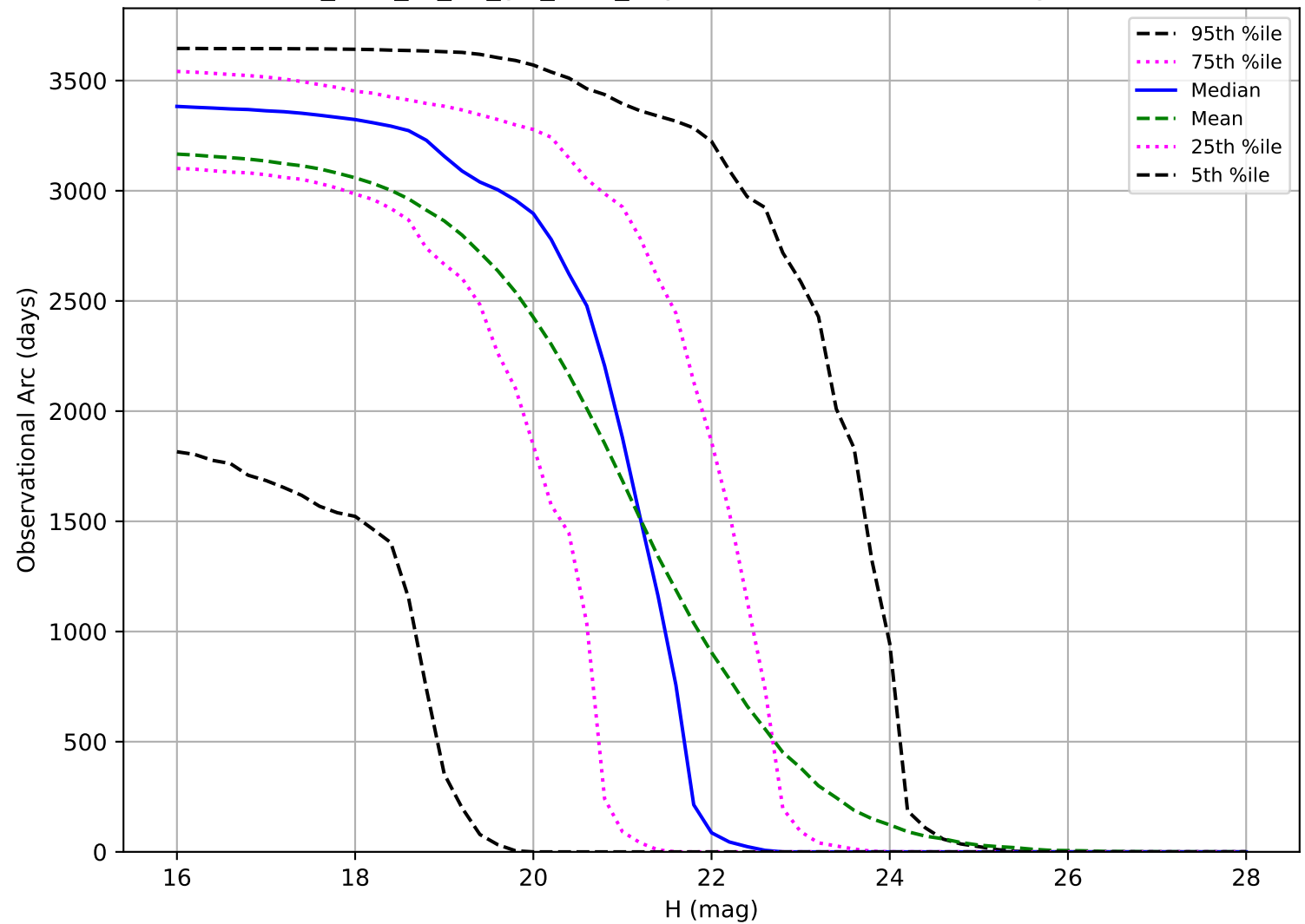
too_elab_r8_d3_giz_v3.4_10yrs: Observational Arc Length NEO
