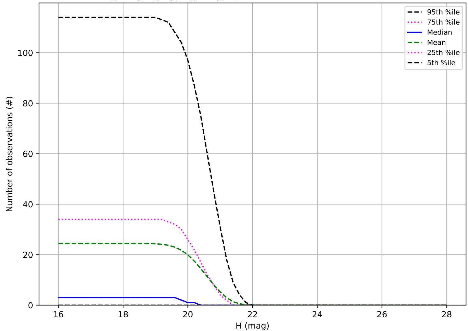
too_elab_r8_d3_giz_v3.4_10yrs: Number of observations Vatira
