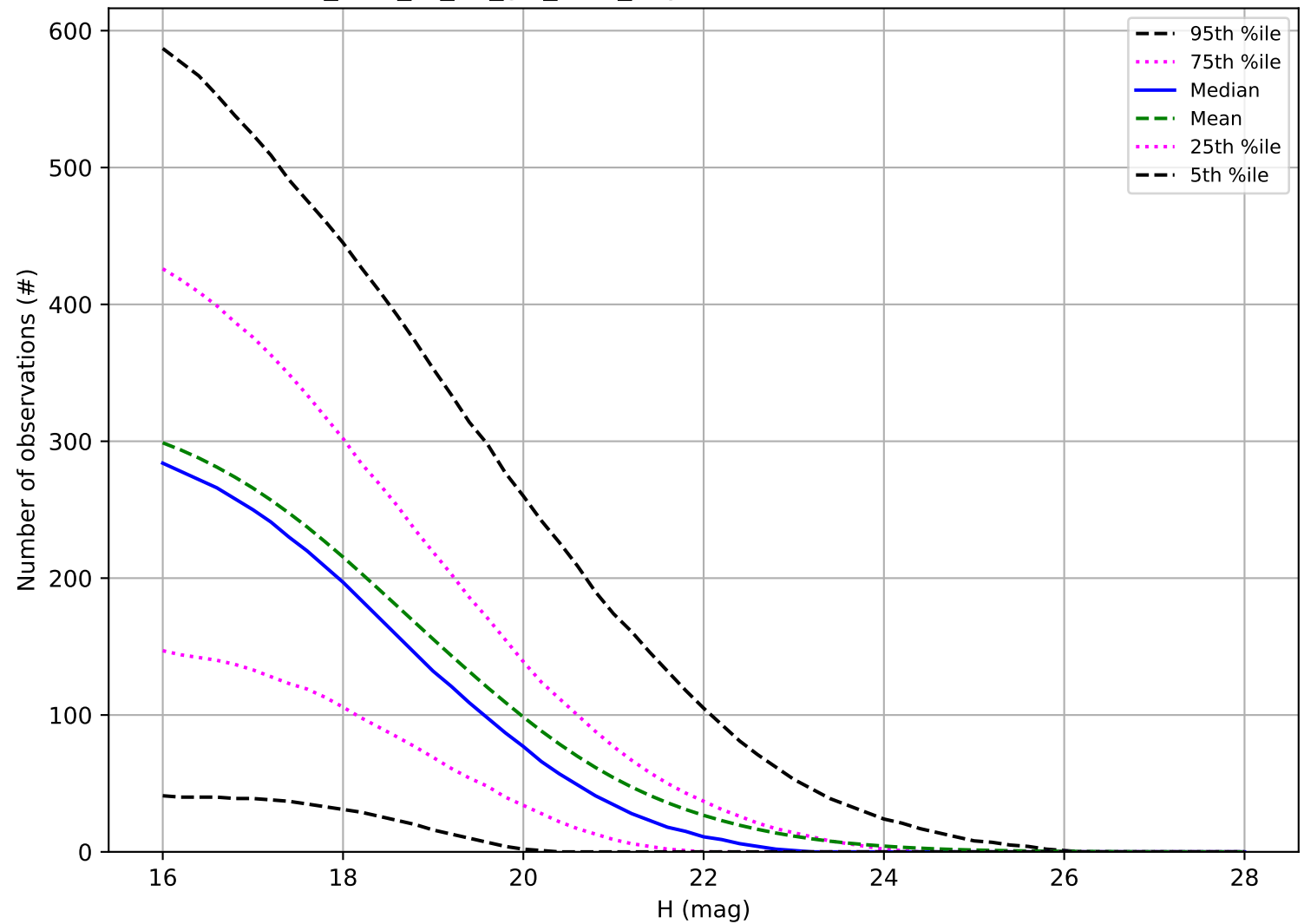
too_elab_r8_d3_giz_v3.4_10yrs: Number of observations PHA
