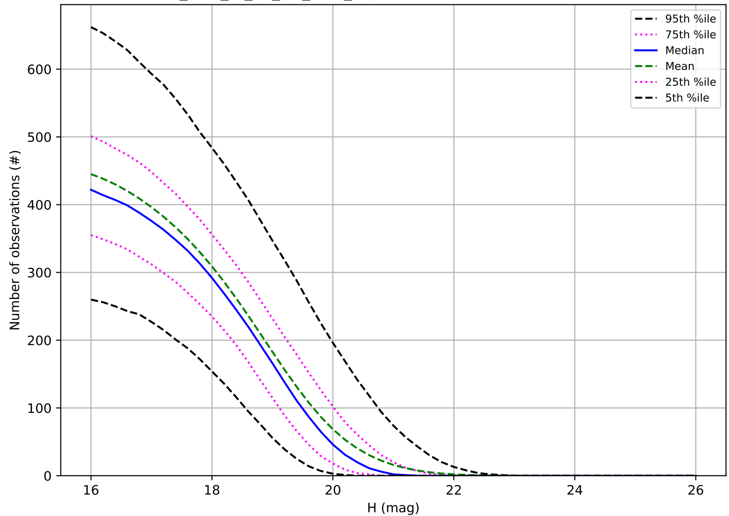
too_elab_r8_d3_giz_v3.4_10yrs: Number of observations MBA
