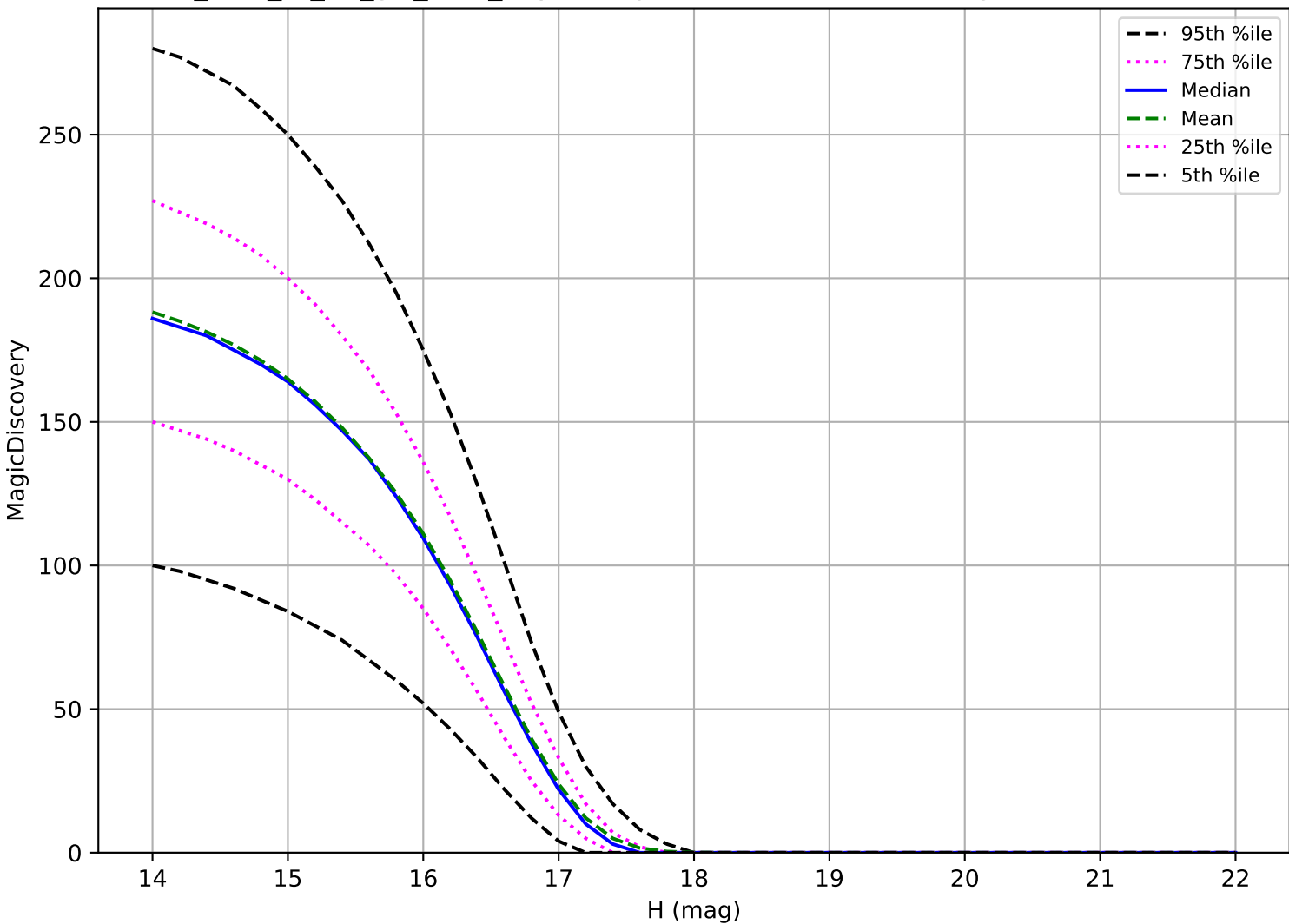
too_elab_r8_d3_giz_v3.4_10yrs: Trojan 6 detections in 60 nights detection loss
