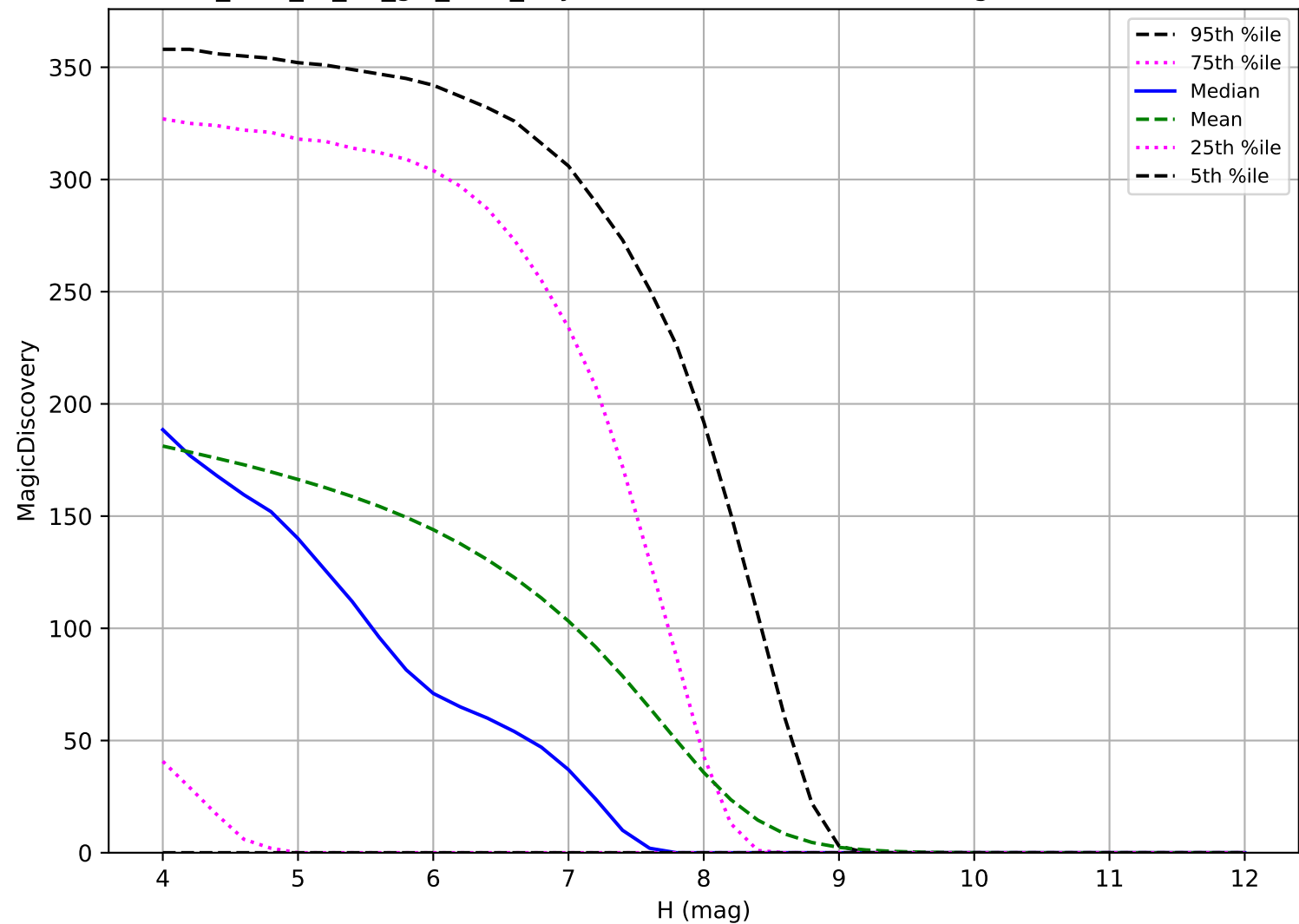
too_elab_r8_d3_giz_v3.4_10yrs: TNO 6 detections in 60 nights detection loss
