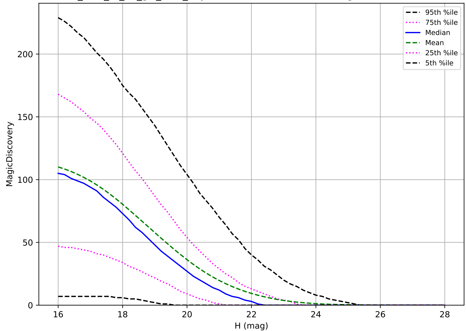
too_elab_r8_d3_giz_v3.4_10yrs: PHA 6 detections in 60 nights detection loss
