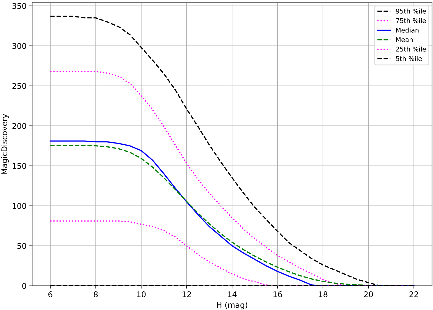
too_elab_r8_d3_giz_v3.4_10yrs: OCC_r5 6 detections in 60 nights detection loss
