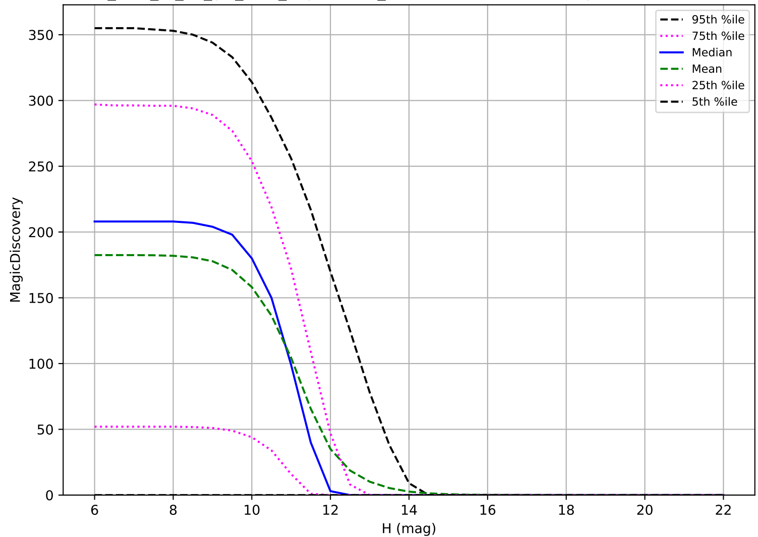
too_elab_r8_d3_giz_v3.4_10yrs: OCC_r20 6 detections in 60 nights detection loss
