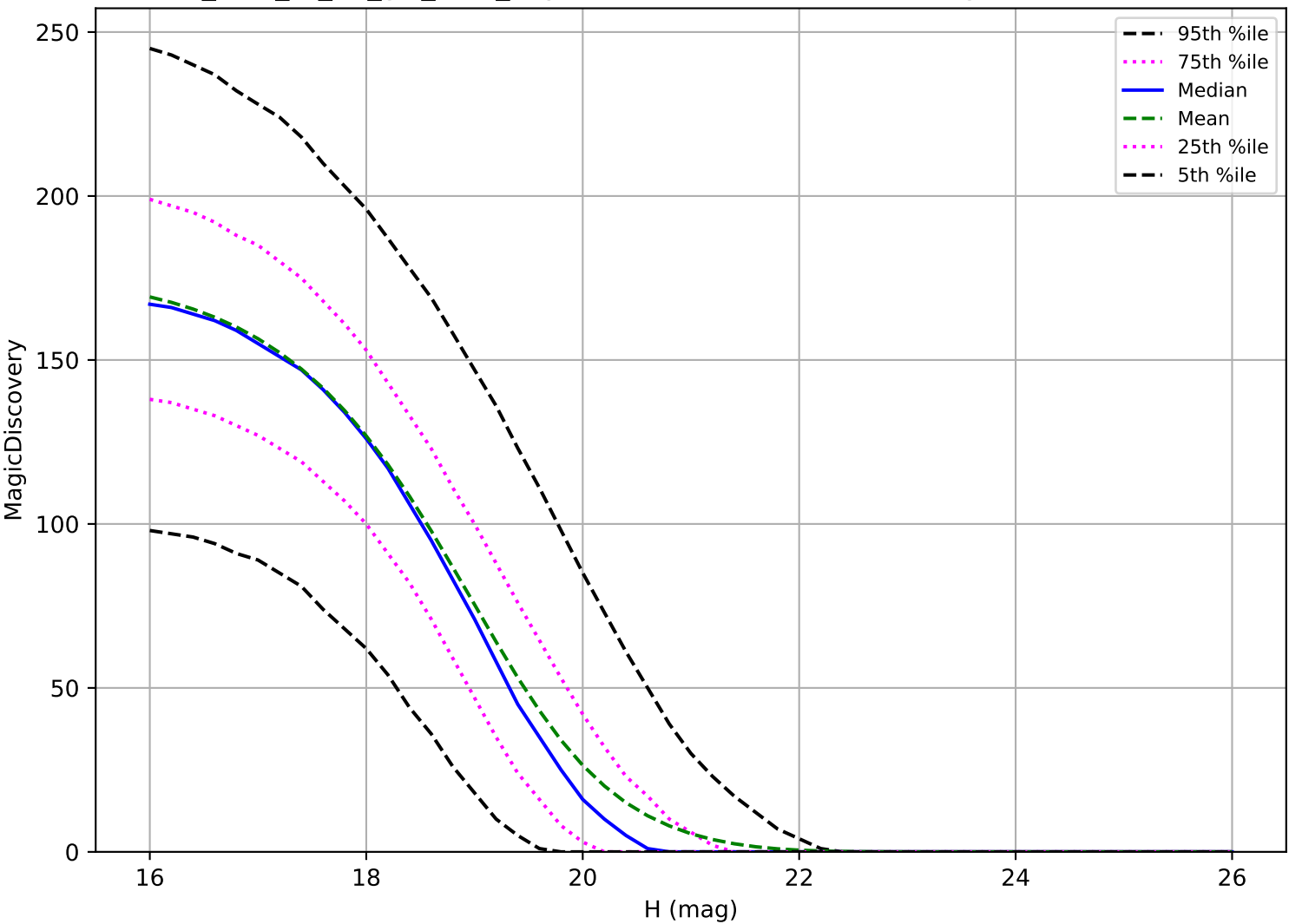
too_elab_r8_d3_giz_v3.4_10yrs: MBA 6 detections in 60 nights detection loss
