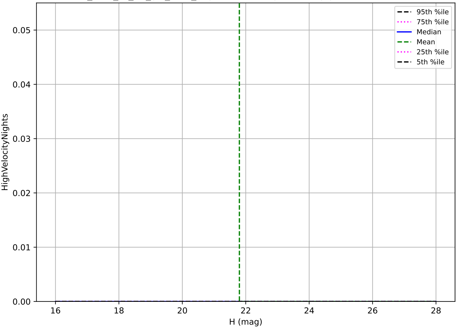
too_elab_r8_d3_giz_v3.4_10yrs: Vatira High velocity pair detection loss
