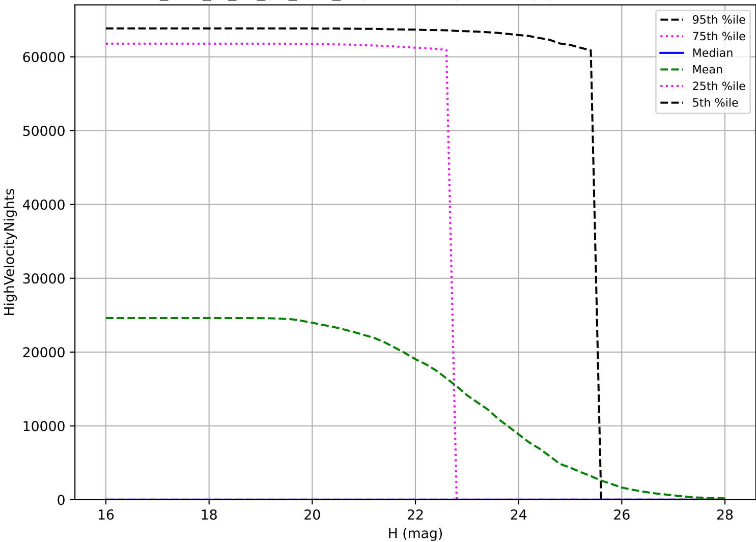
too_elab_r8_d3_giz_v3.4_10yrs: PHA High velocity pair detection loss
