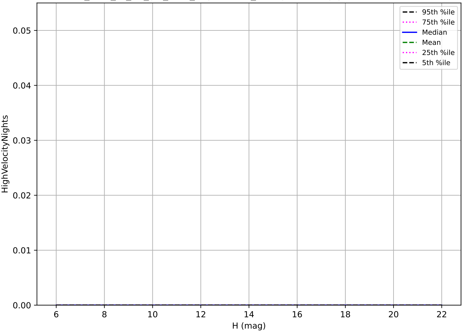
too_elab_r8_d3_giz_v3.4_10yrs: OCC_r5 High velocity pair detection loss
