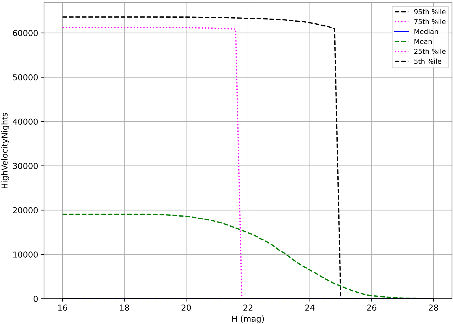
too_elab_r8_d3_giz_v3.4_10yrs: NEO High velocity pair detection loss
