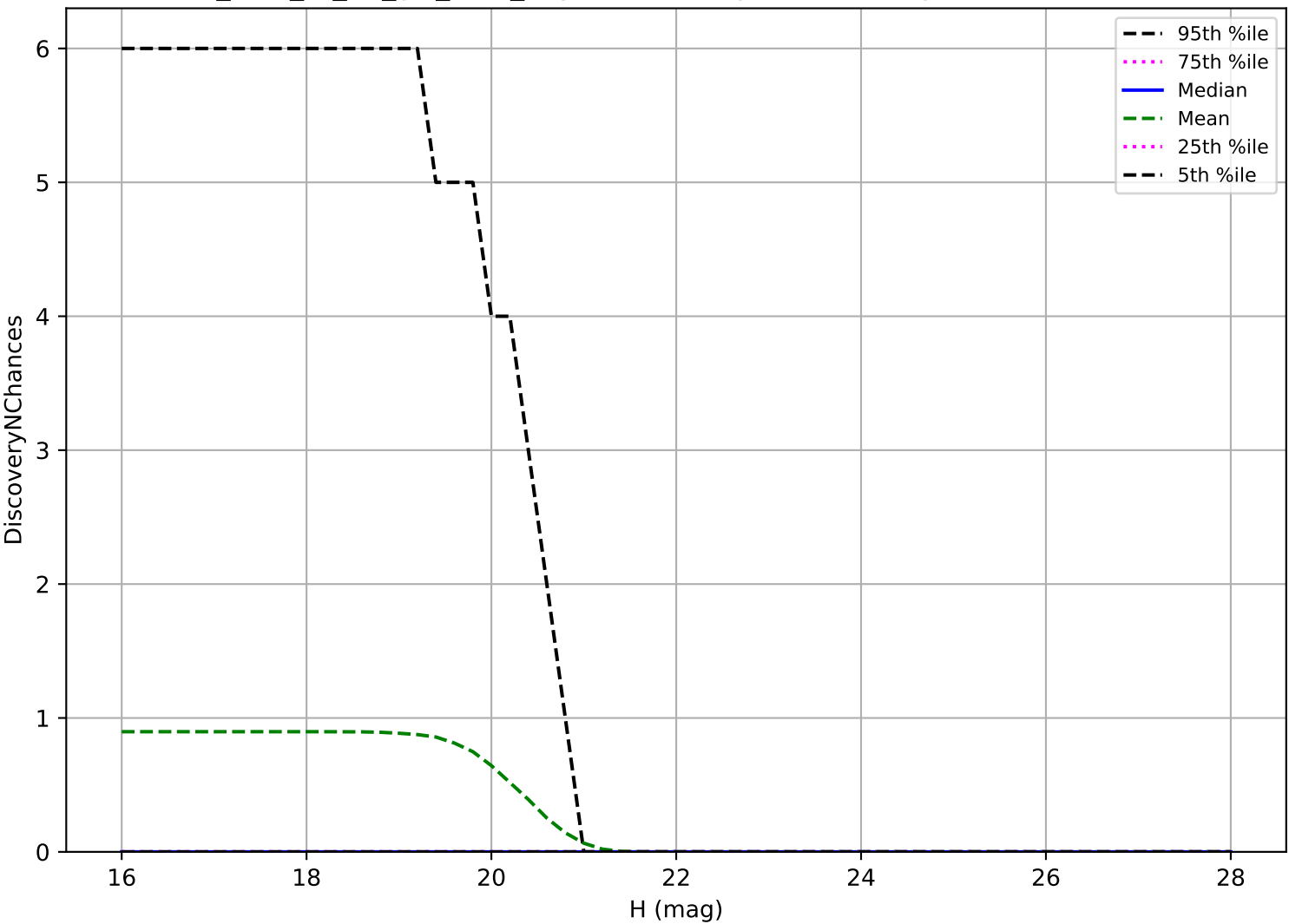
too_elab_r8_d3_giz_v3.4_10yrs: Vatira 3 pairs in 15 nights detection loss
