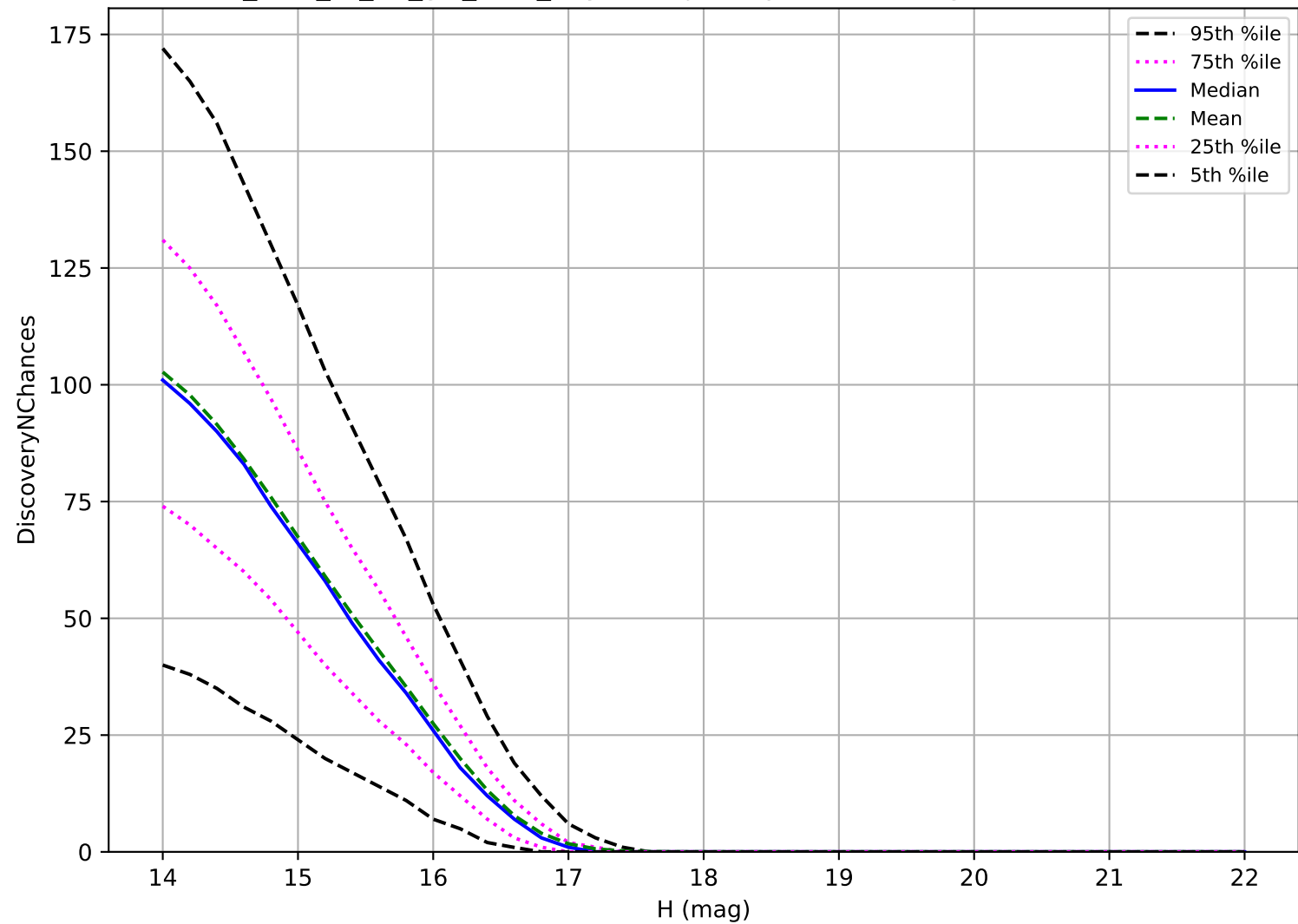
too_elab_r8_d3_giz_v3.4_10yrs: Trojan 3 pairs in 15 nights detection loss
