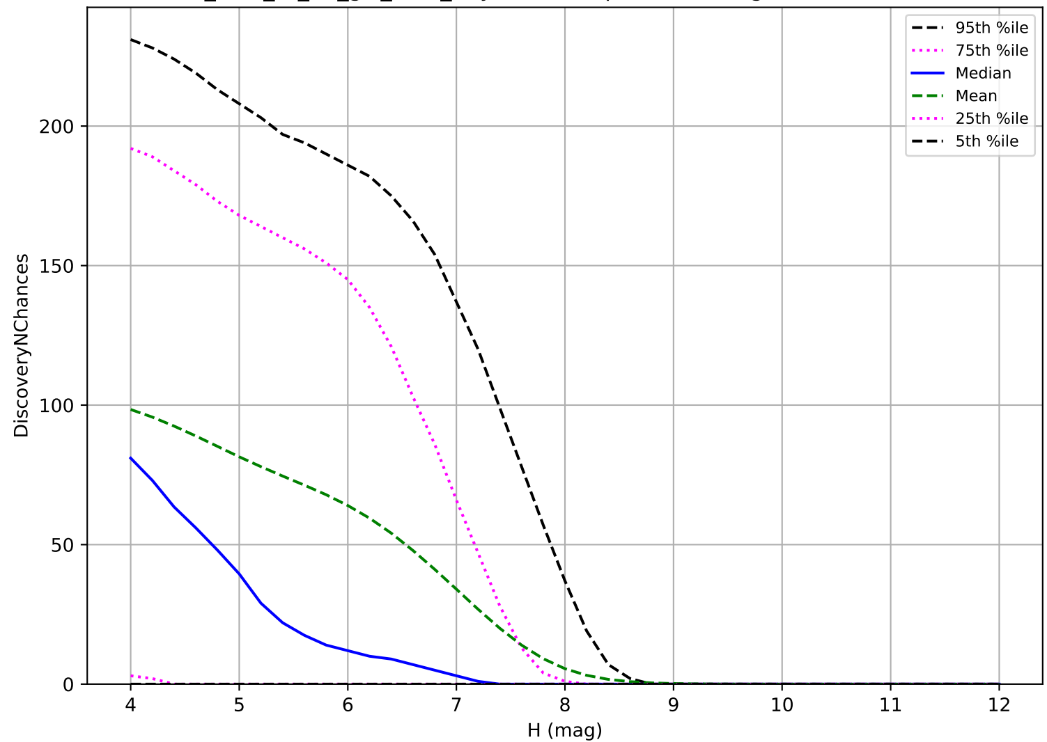
too_elab_r8_d3_giz_v3.4_10yrs: TNO 3 pairs in 15 nights detection loss
