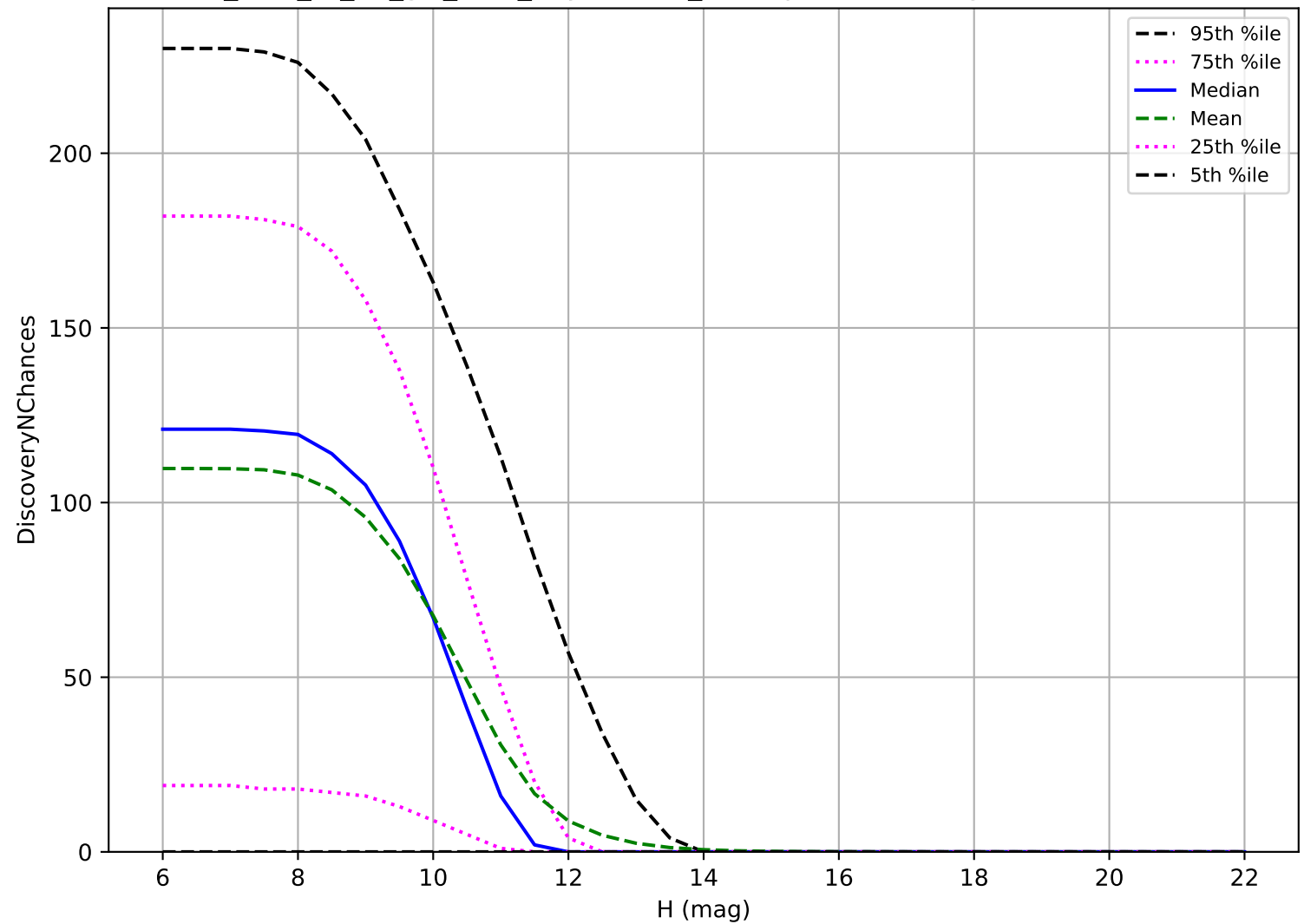
too_elab_r8_d3_giz_v3.4_10yrs: OCC_r20 3 pairs in 15 nights detection loss
