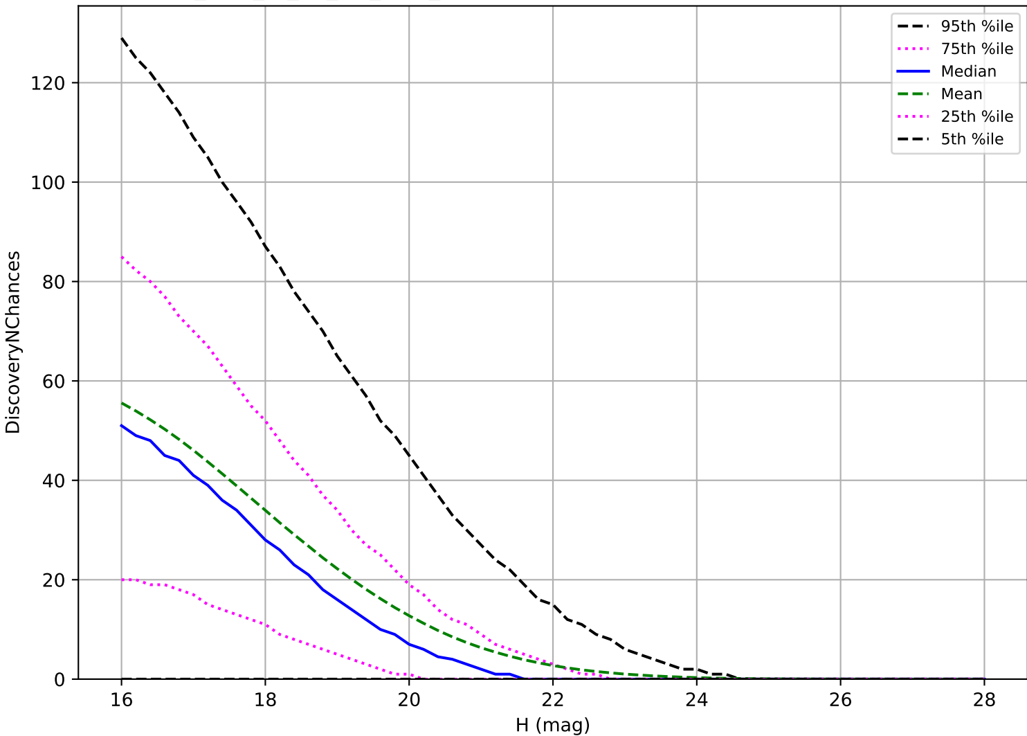
too_elab_r8_d3_giz_v3.4_10yrs: NEO 3 pairs in 15 nights detection loss
