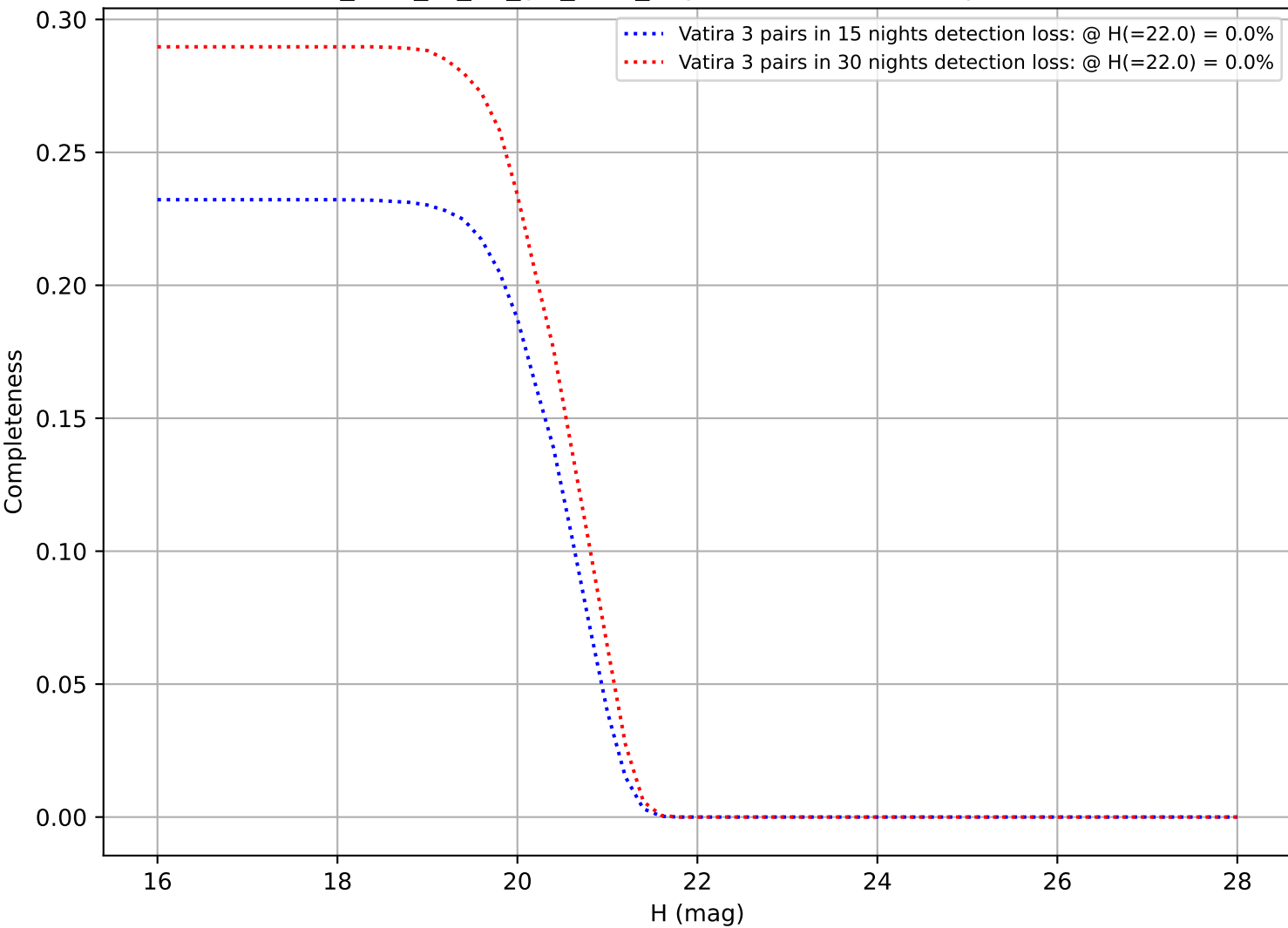
too_elab_r8_d3_giz_v3.4_10yrs: DifferentialCompleteness
