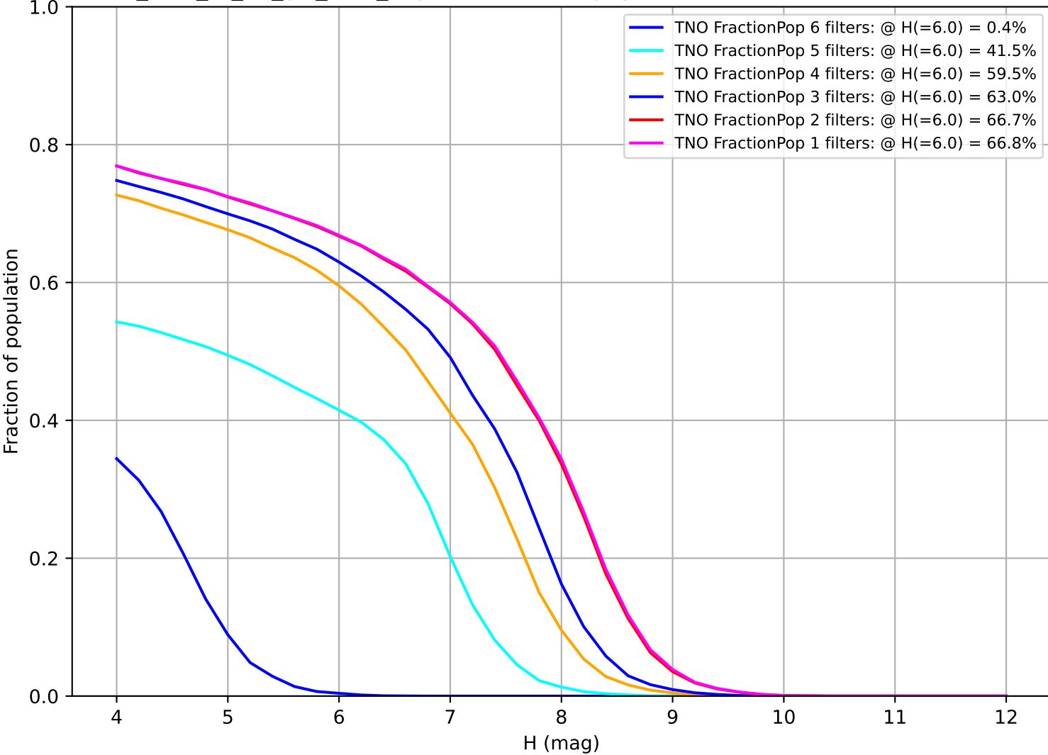
too_elab_r8_d3_giz_v3.4_10yrs: Fraction of population with colors in X filters TNO
