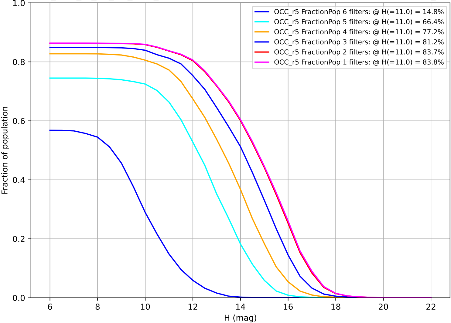
too_elab_r8_d3_giz_v3.4_10yrs: Fraction of population with colors in X filters OCC_r5
