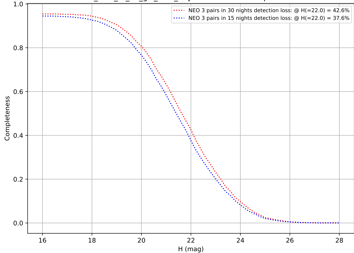
too_elab_r8_d3_giz_v3.4_10yrs: DifferentialCompleteness
