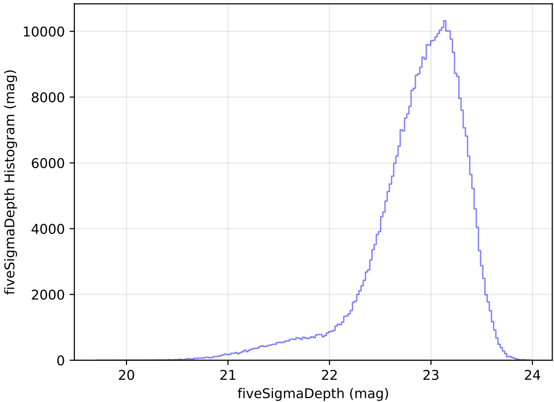
too_elab_r8_d3_giz_v3.4_10yrs z: fiveSigmaDepth Histogram
